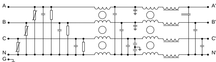
Circuit 1
